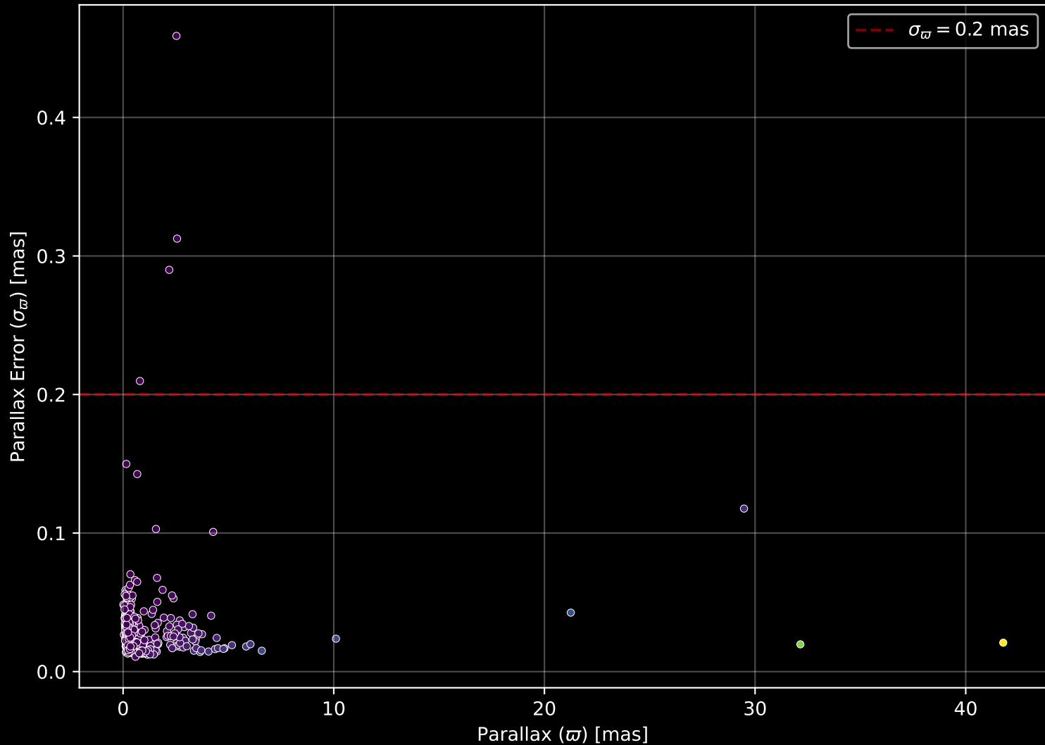
APOGEE DR17 Field: [150+08] Parallax Quality (n= 586)
