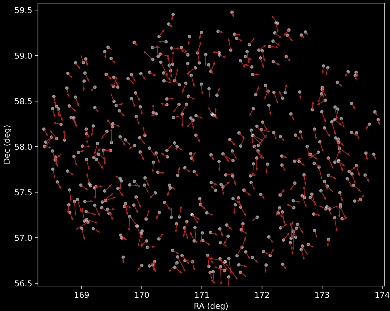
APOGEE DR17 Cluster 6 Proper Motion Vectors (n=407)
