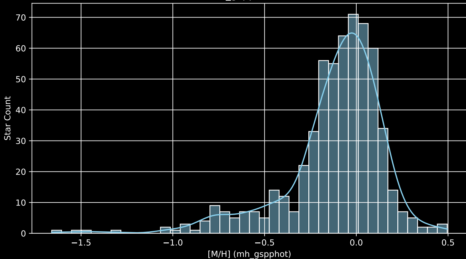
APOGEE DR17 Field: [150+08 [M/H] (mh_gspphot) (n= 584)
