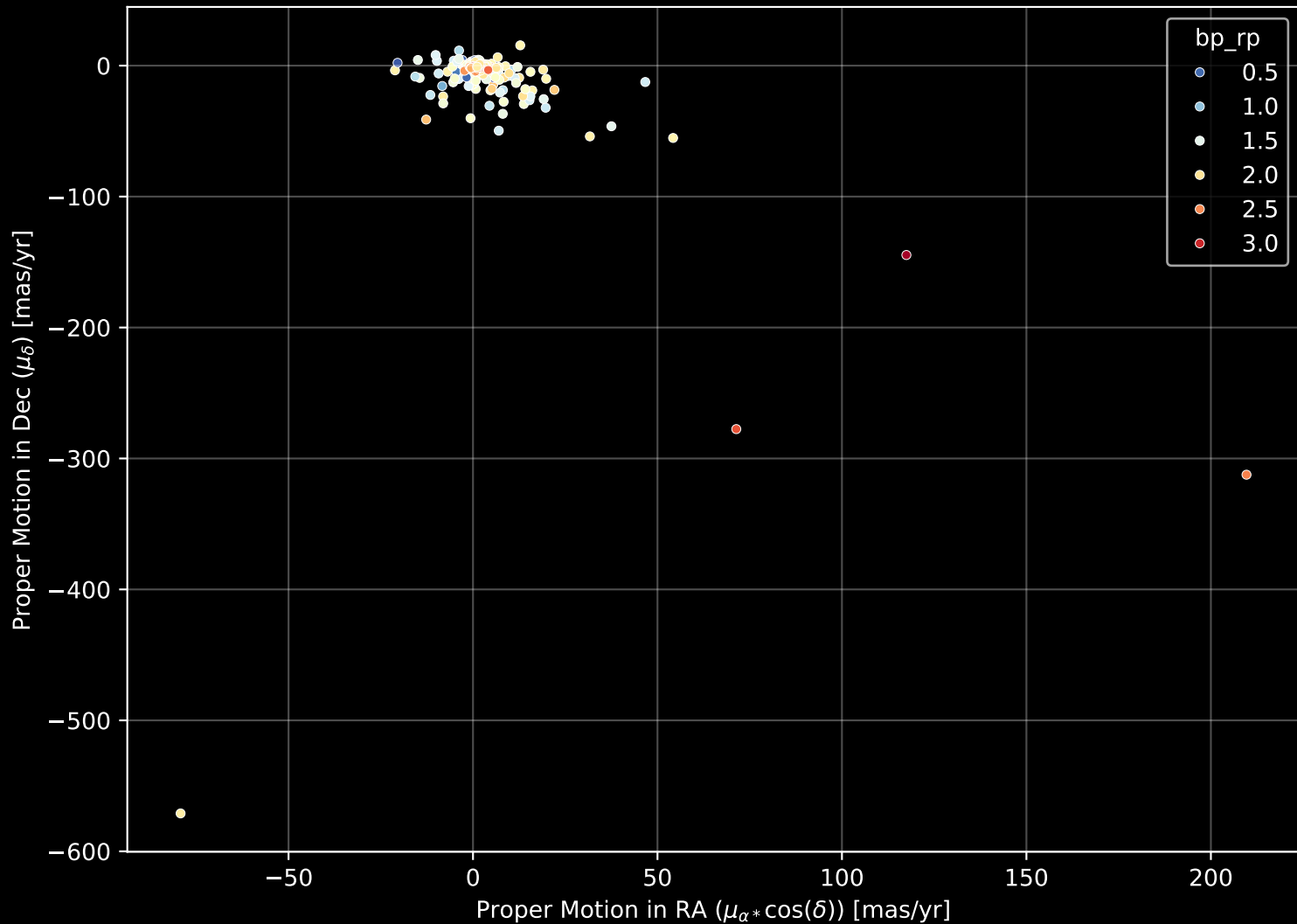
APOGEE DR17 Field: [150+08] Proper Motion Diagram (n= 586)
