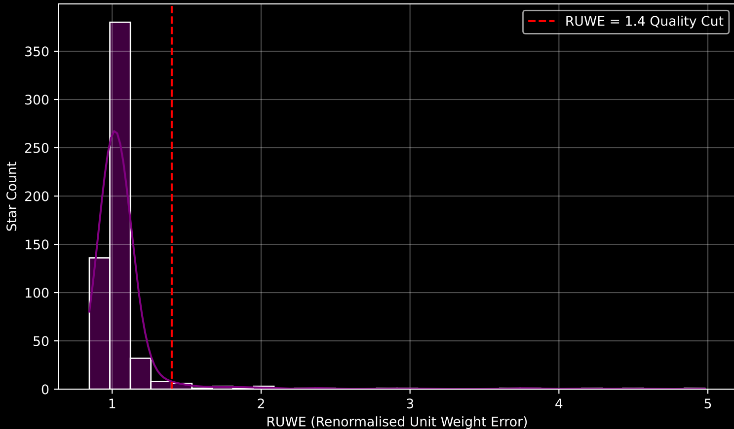
GAPOGEE DR17 Field [150+08] RUWE Distribution (n= 579)
